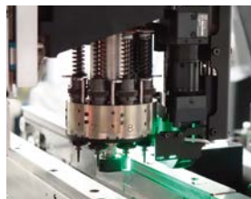
Component side recognition camera
